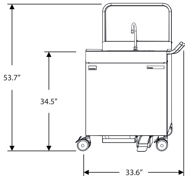
SNK201 - Base Model
