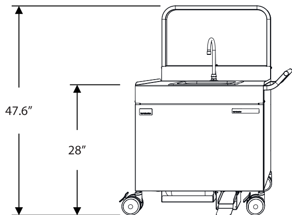
SNK101 - Base Model
