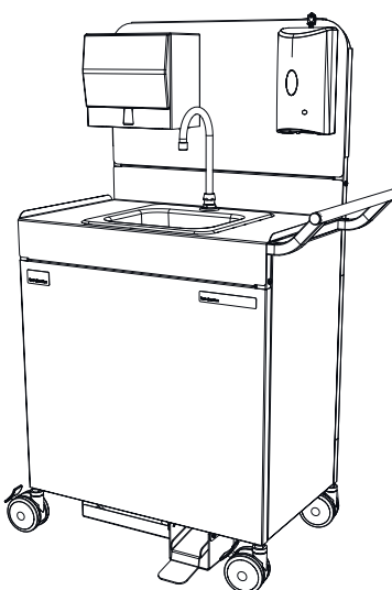
Portable Sink Grades 6+ Counter Height 34-1/2" Premium Model (SNK200)
