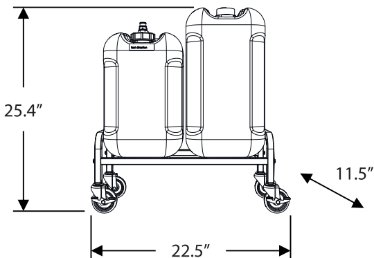
SNK300 - Portable Sink Tank Kit with Dolly (optional accessory)
